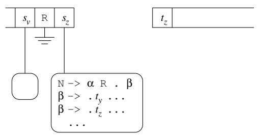
Fig. 3.60: LR error recovery—repairing the input
