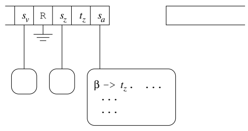
Fig. 3.61: LR error recovery—restarting the parser
