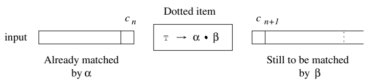
Fig. 2.18: The relation between a dotted item and the input
