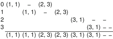
Fig. 2.35: Fitting the strips with entries marked by character
